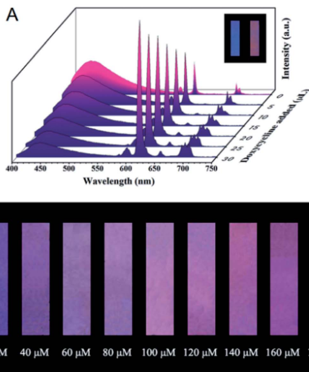
Fig. 8 (A) Fluorescence signal changes of CDs@Eu-MOF after the addition of doxycycline. (B) Fluorescence color change of the test strip after the addition of doxycycline. Reproduced from ref. 50 with the permission from Royal Society of Chemistry.
