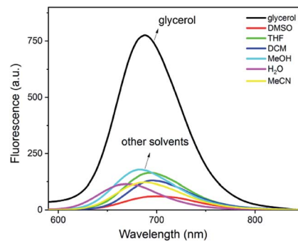
Fig. 2 Fluorescence spectra of DpCy7 (5 \mu\text{M} ) in various freshly prepared solvents. The solvents included: DMSO, tetrahydrofuran, dichloromethane, methanol, H 2 O, acetonitrile and glycerol.
