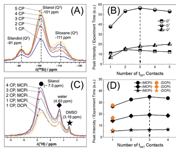
Fig. 3 Optimization of the number of CP contacts of MCPi experiment for the DMSO- h_6 -adsorbed SiNP. (A) \{^1\text{H}-^{29}\text{Si}\}^{-1}\text{H} MultiCP: \text{RD} = 4.0 s, contact time = 5 ms. (B) Evolution of ^{29}\text{Si} intensity with the number of contacts in ^{29}\text{Si} MultiCP experiment. (C) \{^1\text{H}-^{29}\text{Si}\}^{-1}\text{H} MCPi and DCPI spectra ( \text{RD} = 4.0 s, t_{\text{cp1}} = t_{\text{cp2}} = 5 ms). (D) Evolution of ^1\text{H} intensity with the number of contacts in MCPi and DCPI experiments.
