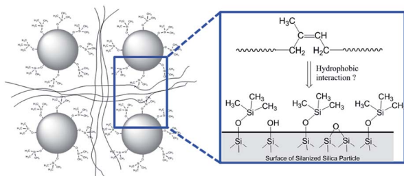
Fig. 5 Schematic representation of the silica surface in a polymer-silica composite, where the silica has been silanized by trimethylchlorosilane and the polymer is polyisoprene (see Experimental).
