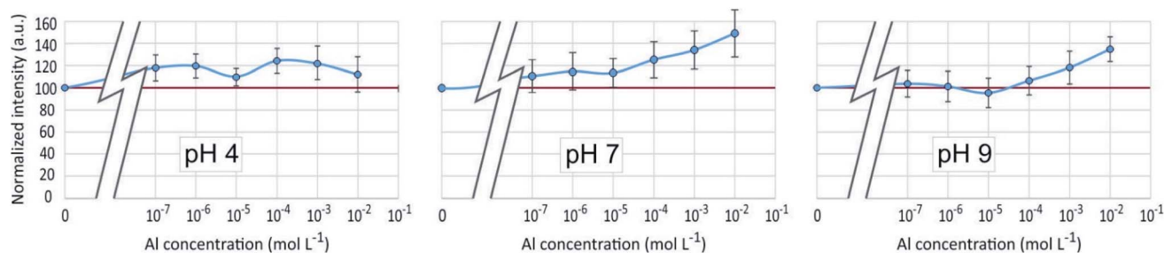
Fig. 8 Fluorescence intensity at \lambda_{\text{ex}} = 330 nm, \lambda_{\text{em}} = 510 nm of the PDMPO –Al system at various pH as a function of the concentration of Al in \text{mol L}^{-1} .
