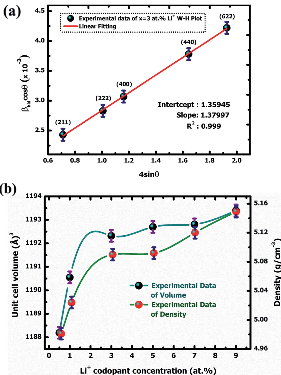
Fig. 2 W–H plot of Y_2O_3:4 at% Eu^{3+} , xLi^+ (a) x = 3 at% nanophosphor (b) variation of unit cell volume and density with Li^+ codoping concentration.
