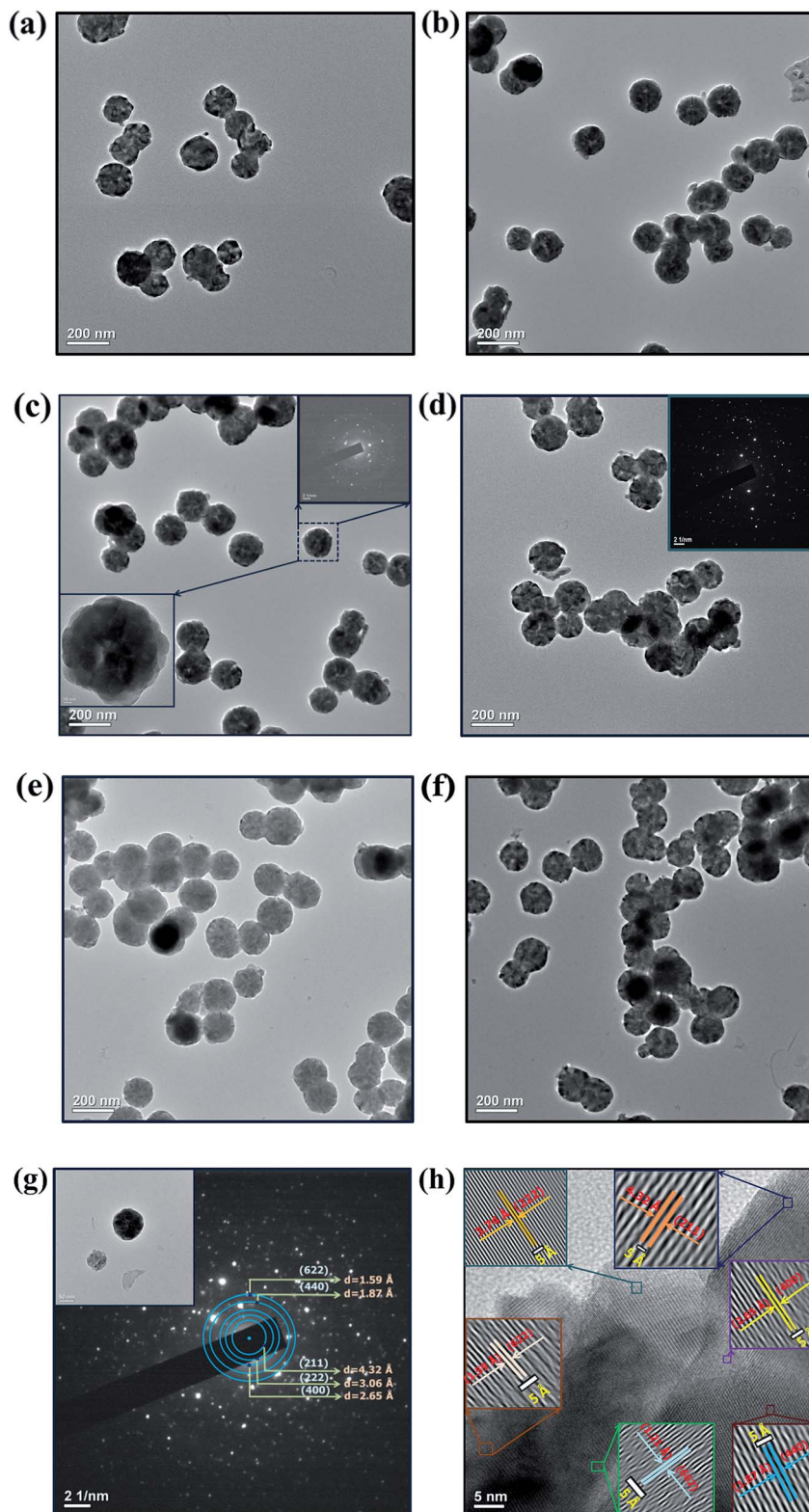
Fig. 6 HR-TEM Images of Y 2 O 3 :4 at% Eu 3+ , xLi + (a) x = 0.5 at%, (b) x = 1 at%, (c) x = 3 at%, (d) x = 5 at%, (e) x = 7 at%, (f) x = 9 at% nanophosphors. (g) The magnified HR-TEM image and SAED pattern analysis of x = 9 at% prepared crystalline sample. (h) Lattice fringes of x = 9 at% samples corresponds to cubic yttrium(III) oxide (Y 2 O 3 ).
