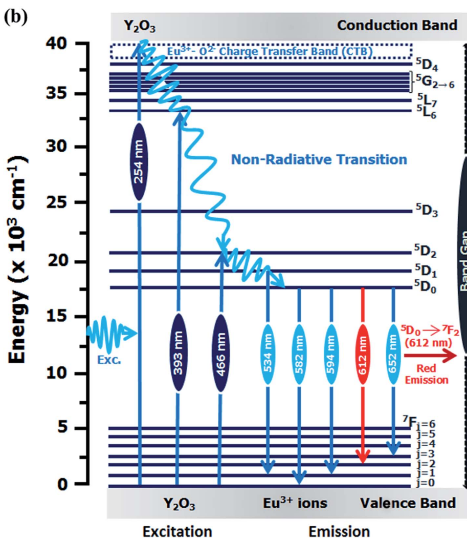
Fig. 9 (a) PL lifetime decay curves of \text{Y}_2\text{O}_3:4 \text{ at}\% \text{Eu}^{3+}, x\text{Li}^+ ( x = 0.5, 1, 3, 5, 7, 9 \text{ at}\% ) nanophosphors. (b) Schematic energy level diagram for \text{Y}_2\text{O}_3:4 \text{ at}\% \text{Eu}^{3+}, x\text{Li}^+ ( x = 0.5, 1, 3, 5, 7, 9 \text{ at}\% ) nanophosphors.
