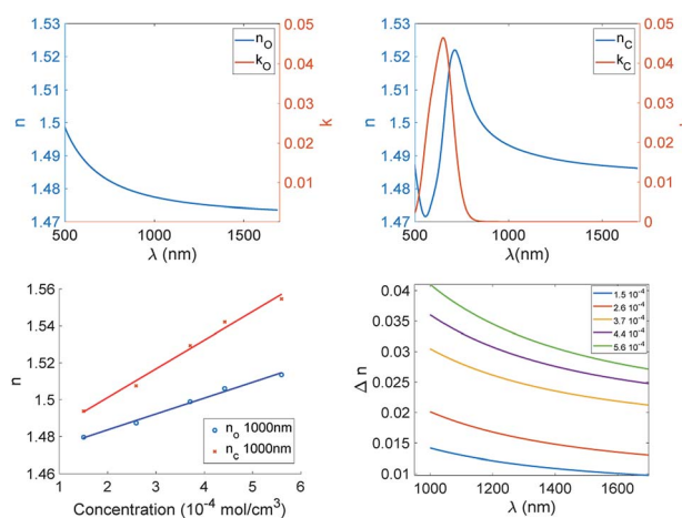
Fig. 7 Top: Complex refractive index for the open (left panel) and closed (right panel) forms of the AmAm doped CAB film (the plots of the other two derivatives are reported in Fig. S5†). Bottom: (left panel) The real part of the refractive index at 1000 nm in the open and closed forms as a function of the molar concentration of AmAm in CAB; (right panel) refractive index difference ( \Delta n = n_c - n_o ) as function of the wavelength.
