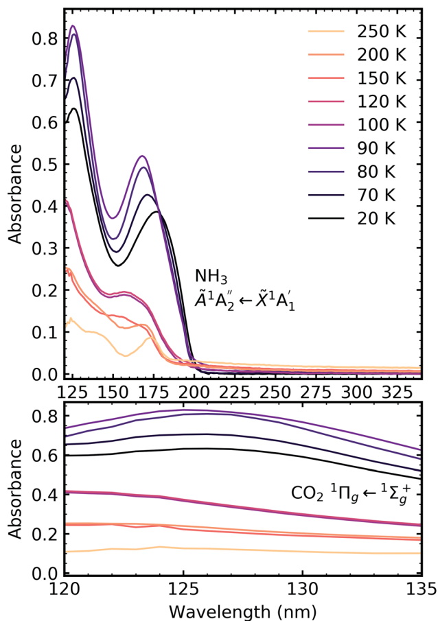
Fig. 9 VUV spectra of the thermal processing of a 1 : 3 CO 2 : NH 3 mixture from 20–200 K between 120–340 nm (top plot). Bottom plot shows the lack of vibrational structure of the CO 2 ^1\Pi_g \leftarrow ^-1\Sigma_g^+ transition between 120–135 nm.
