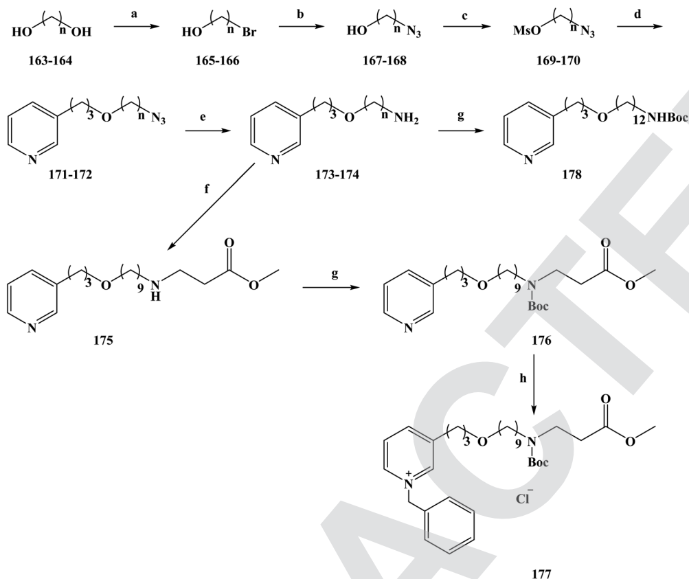
Scheme 8 Synthesis of the oxygenated 3-alkylpyridine marine alkaloid analogue compounds 177 and 178 . Reagents and conditions: (a) HBr (aq), toluene, reflux; (b) \text{NaN}_3 , DMSO, r.t., 12 h; (c) MsCl, \text{Et}_3\text{N} , methylene chloride, stirring, 3 h; (d) NaOH, \text{Bu}_4\text{N}^+\text{Br}^- ; (e) \text{LiAlH}_4 , THF; (f) methyl acrylate, toluene, reflux; (g) \text{Boc}_2\text{O} , methylene chloride; (h) \text{BnCl} , reflux.
