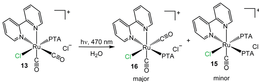
Scheme 11 Light-induced isomerization ( \lambda = 470\text{ nm} , 72 h) of cis,trans -[Ru(bpy)(CO) 2 Cl(PTA)]Cl ( 13 ) to cis,cis -[Ru(bpy)(CO) 2 Cl(PTA)]Cl ( 16 ) and cis,cis -[Ru(bpy)Cl(CO)(PTA) 2 ]Cl ( 15 ).
