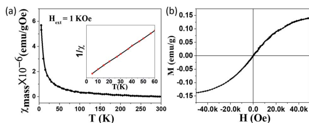
Fig. 3 Magnetic properties of GO measured by PPMS. (a) Typical \chi-T curve measured from 5 to 300 K under the extra field H = 1 kOe. Inset is the corresponding 1/\chi - T curve. (b) M-H curve measured at 5 K.
