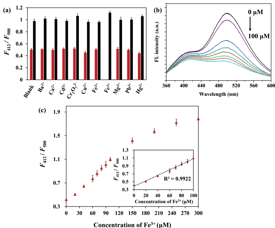
Fig. 4 (a) Selectivity of CSCDs@DC (0.4 mg mL -1 ) aqueous solution for Fe 3+ ions over other metal ions. The red bars represented the addition of metal ions (100 \mu M for all the metal ions). The black bars represented the subsequent addition of 100 \mu M Fe 3+ to the CSCDs@DC aqueous solution. (b) FL spectra of CSCDs@DC (0.4 mg mL -1 ) with different concentrations of Fe 3+ ions at 330 nm. (c) FL emission ratios ( F_{412}/F_{500} ) of CSCDs@DC (0.4 mg mL -1 ) in the presence of different Fe 3+ ions concentrations in the range from 0 \mu M to 300 \mu M. Inset is linear relationship between F_{412}/F_{500} and Fe 3+ ions concentration in the range from 0 \mu M to 100 \mu M.
