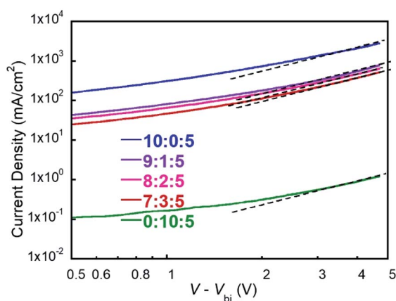
Fig. 5 J - V curves of devices with different polymer ratios.
