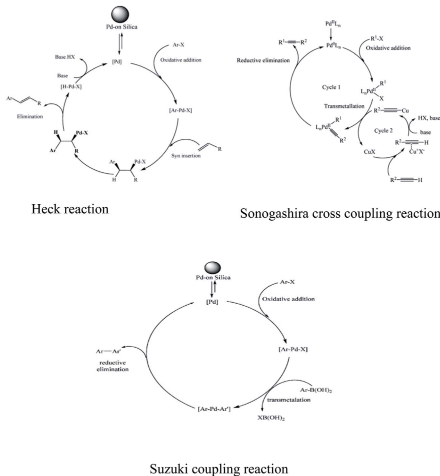
Fig. 6 Schematic representation of Heck Article reaction, Sonogashira cross coupling, and Suzuki coupling reaction. Reprinted with permission from ref. 52.
