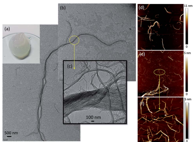
Fig. 1 (a) Visual appearance, (b and c) TEM micrograph and ((d) 20 \times 20 \mu\text{m} ; (e) 3 \times 3 \mu\text{m} ; (f) 1 \times 1 \mu\text{m} ) AFM images of as-prepared ChNF.
