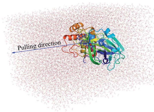
Fig. 1 Initial conformation of FPL simulations of the SARS-CoV-2 Mpro + periandrin V .
