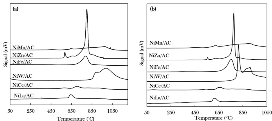
Fig. 3 Temperature-programmed desorption patterns of (a) TPD- \text{NH}_3 and (b) TPD- \text{CO}_2 of binary metal oxide-supported AC catalysts.
