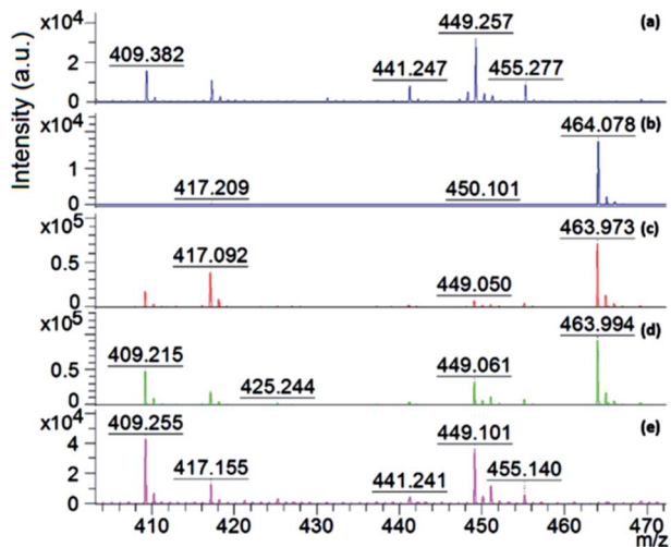
Fig. 11 Comparison of the average mass spectra of: (a) 9aa (matrix), (b) initial AR1 solution; and aqueous solution after AR1 degradation with (c) 0.05 M H 2 O 2 , (d) 0.1 M H 2 O 2 , and (e) 0.2 M H 2 O 2 .
