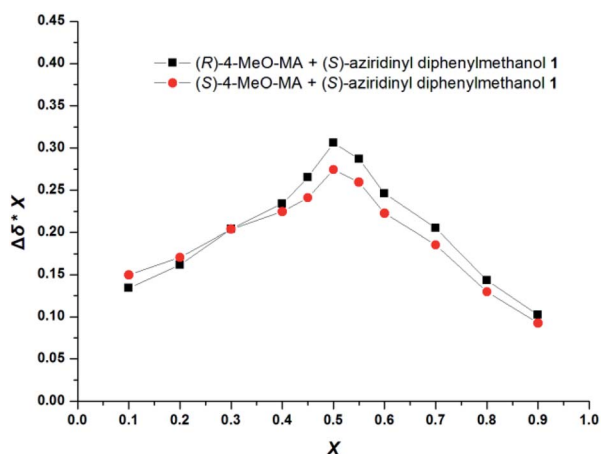
Fig. 3 Job plots of ( S )-aziridinyldiphenylmethanol 1 with ( R )-4-MeO-MA and ( S )-4-MeO-MA. \Delta\delta stands for the chemical shift change of the \alpha -H proton of ( R )- and ( S )-4-MeO-MA in the presence of ( S )-aziridinyldiphenylmethanol 1 . X stands for the molar fraction of the ( S )-aziridinyldiphenylmethanol 1 ( X = [(\text{S})\text{-aziridinyldiphenylmethanol } \mathbf{1}] / [(\text{S})\text{-aziridinyldiphenylmethanol } \mathbf{1}] + [4\text{-MeO-MA}] ). The total concentration is 10 mM in \text{CDCl}_3 .
