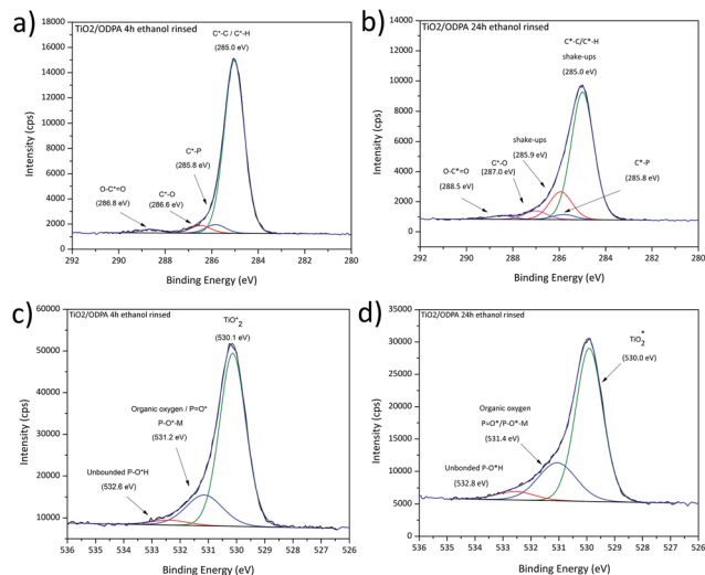
Fig. 5 High-resolution C1s and O1s XPS spectra obtained for ODPAs layers on titania after immersion in ODPAs solution for 4 h (a) and (c); 24 h (b) and (d).
