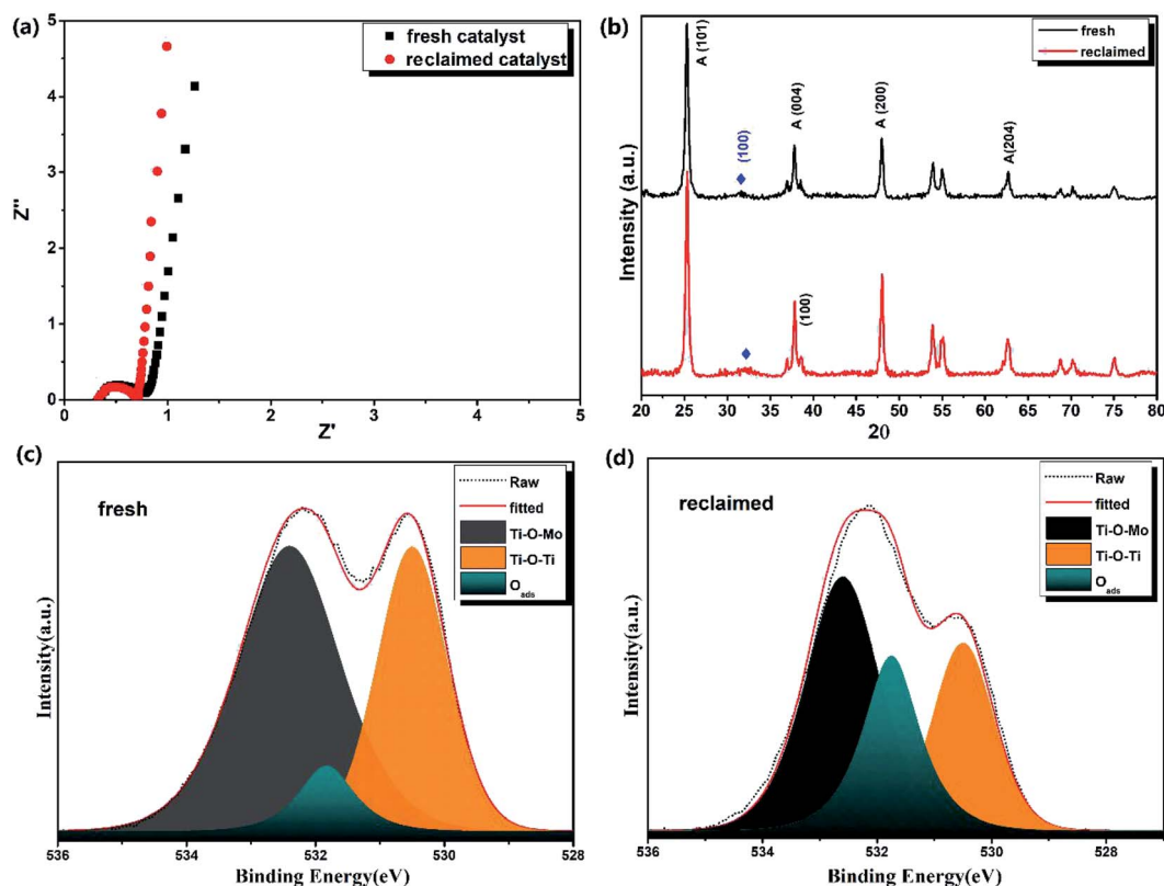
Fig. 6 EIS spectra (a) XRD patterns (b) of the fresh \text{MoS}_2\text{@TNr} catalyst and the reclaimed catalyst after the piezoelectric degradation process. Comparison of O 1s orbital peaks of fresh \text{MoS}_2\text{@TNr} catalyst (c) and the reclaimed \text{MoS}_2\text{@TNr} composites (d).
