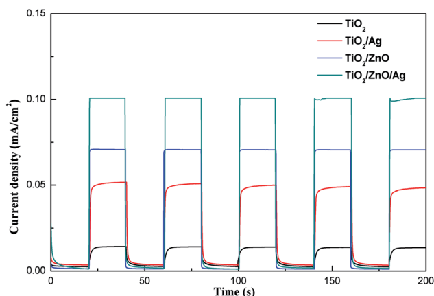
Fig. 7 Transient photocurrent responses of different samples.
