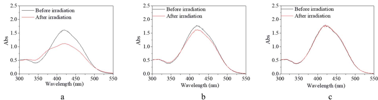
Fig. 8 UV-vis spectra of the copolymer solution before and after irradiation by blue light with a light density of 1000 lux. (a) 95% DMSO and 5% water; (b) 90% DMSO and 10% water; (c) 85% DMSO and 15% water.
