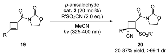
Scheme 7 p -Anisaldehyde catalyzed sulfonylcynylation of chiral cyclobutenes.
