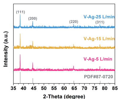
Fig. 3 XRD patterns of V-Ag- 5 \text{ L min}^{-1} , V-Ag- 15 \text{ L min}^{-1} , and V-Ag- 25 \text{ L min}^{-1} samples.
