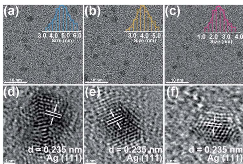
Fig. 2 Characterization of V-Ag nanoparticles at different carrier gas flow rates. Low-magnification TEM images and high-resolution TEM images for (a and d) 5 \text{ L min}^{-1} , (b and e) 15 \text{ L min}^{-1} and (c and f) 25 \text{ L min}^{-1} , the insets are corresponding the size distribution.
