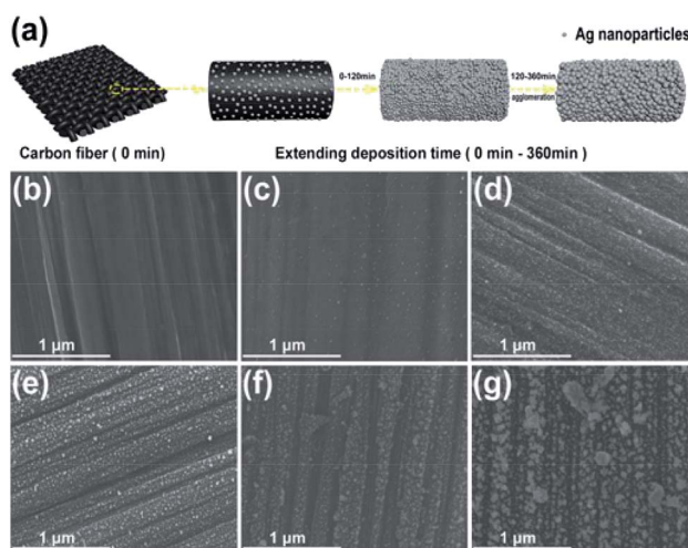
Fig. 4 (a) A schematic of the deposition process of Ag nanoparticles on the carbon fiber with the extension of deposition time. SEM images of V-Ag nanoparticles ( 5 \text{ L min}^{-1} ) deposited on the carbon fiber at different deposited time with a blank carbon fiber as a reference. (b) Blank carbon fiber. (c) 30 min. (d) 60 min. (e) 120 min. (f) 240 min. (g) 360 min.
