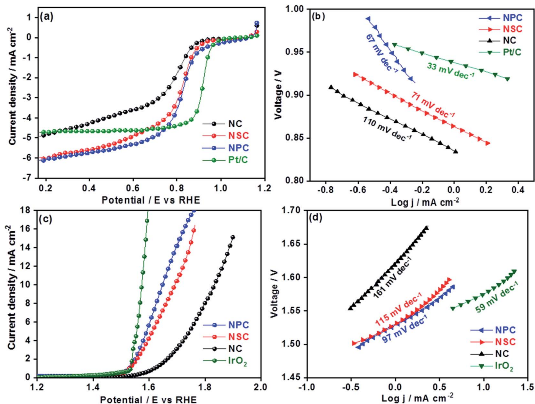
Fig. 4 (a) Cathodic linear sweep voltammograms of NSC, NPC, NC and Pt/C at 1600 rpm in 0.1 M KOH oxygen saturated solution (b) Tafel slopes from the cathodic linear sweep voltammograms (c) anodic linear sweep voltammograms of NC, NSC, NPC and IrO 2 catalysts at 1600 rpm. (d) Tafel slopes from obtained anodic linear sweep voltammograms.
