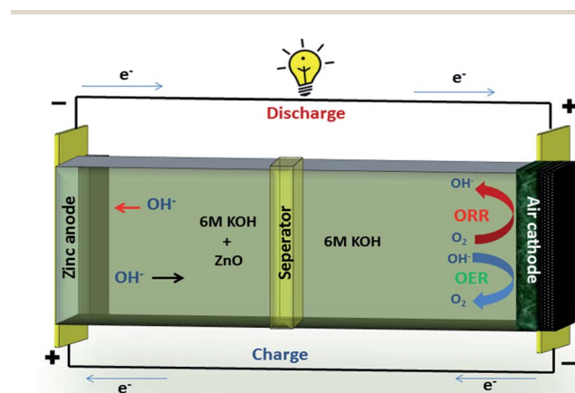
Fig. 7 Zinc-air schematic.
