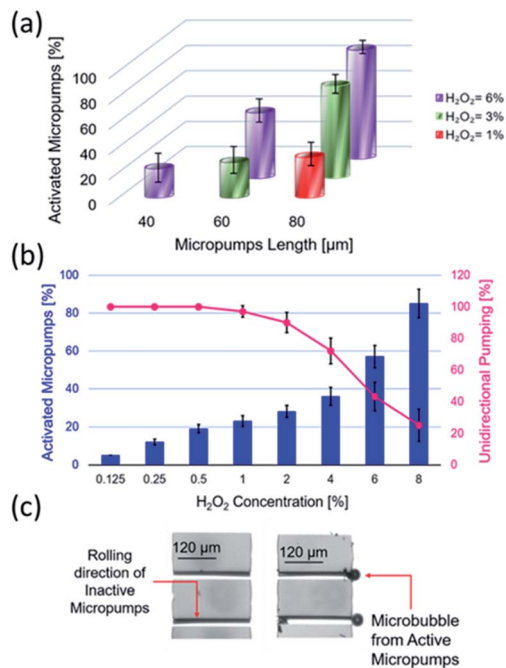
Fig. 2 Characterization of Ti/FeNi/Pt microtubes in a hydrogen peroxide solution. (a) Population of active microtubes (generating O_2 bubbles) with lengths 40, 60 and 80 \mu\text{m} immersed in H_2O_2 1% v/v (red colour), 3% v/v (green colour), and 6% v/v (purple colour), respectively. (b) The population of activated microtubes with 120 \mu\text{m} length. Percentages of active microtubes with 120 \mu\text{m} length in unidirectional (bubbles' ejection from one tubular opening) and overloaded (bubbles' ejection from both tubular openings) regimes. (c) Optical microscopy image of inactive microtubes ( i.e. , generating molecular oxygen, O_2 microbubbles are absent) and active tubes ( i.e. , producing visible O_2 microbubbles).
