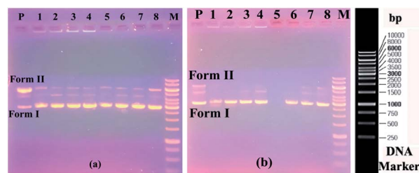
Fig. 1 Electrophoresis images of pBR322 plasmid DNA interacting with compounds. P: only plasmid DNA, M: DNA marker. (a) Compound 4, 1→4: 10\,000\ \mu\text{M} , 5000\ \mu\text{M} , 2500\ \mu\text{M} , 1250\ \mu\text{M} ; 5→8: only solvent (DMF) 100%, 50%, 25% and 12.5%. (b) Compound 5, 1→4: 10\,000\ \mu\text{M} , 5000\ \mu\text{M} , 2500\ \mu\text{M} , 1250\ \mu\text{M} ; compound 6, 5→8: 10\,000\ \mu\text{M} , 5000\ \mu\text{M} , 2500\ \mu\text{M} , 1250\ \mu\text{M} . (c) Standard DNA marker (1 Kb DNA ladder).
