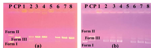
Fig. 5 Electrophoresis images of compound-pBR322 plasmid DNA mixture after interactions with the enzymes Bam HI (a) and Hind III (b). P: plasmid DNA, CP: cut plasmid DNA, compound 7, 1→4: 10 000 \mu\text{M} , 5000 \mu\text{M} , 2500 \mu\text{M} , 1250 \mu\text{M} ; compound 11, 5→8: 10 000 \mu\text{M} , 5000 \mu\text{M} , 2500 \mu\text{M} , 1250 \mu\text{M} .
