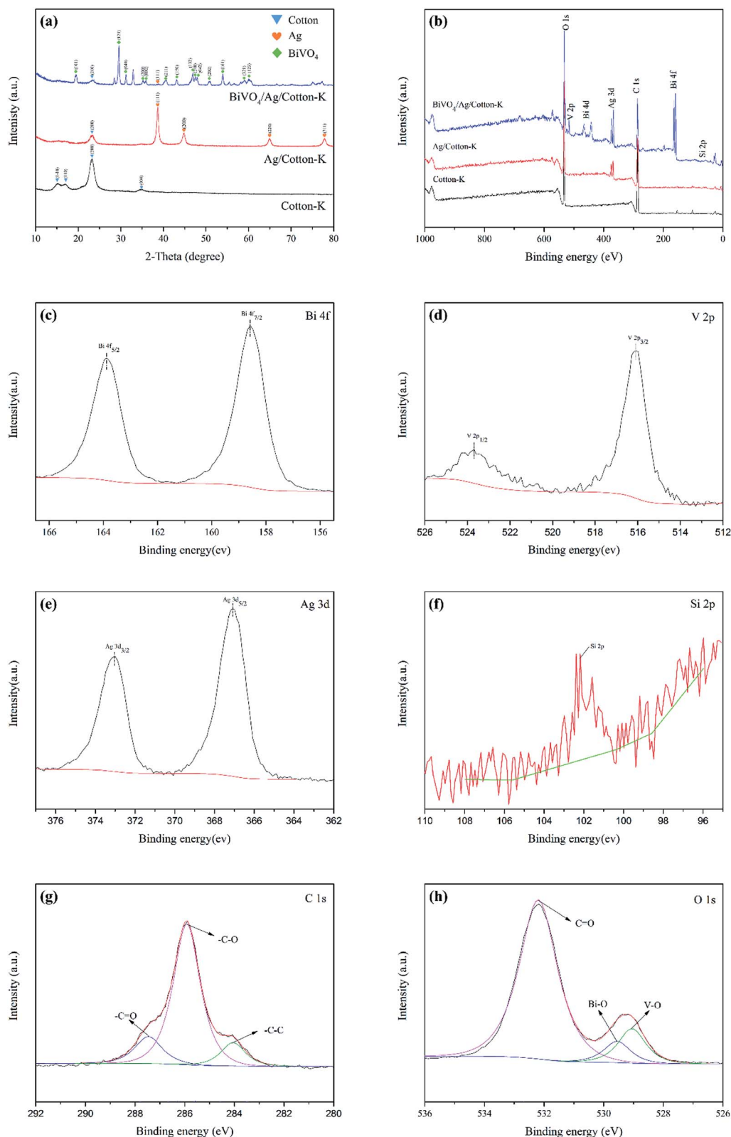
Fig. 3 (a) XRD patterns of cotton-K, Ag/cotton-K, \text{BiVO}_4/\text{Ag}/\text{cotton-K} . (b) XPS survey spectra. High resolution XPS spectrum of (c) Bi 4f; (d) V 2p; (e) Ag 3d; (f) Si 2p; (g) C 1s; (h) O 1s.
