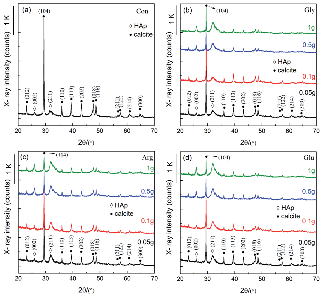
Fig. 1 XRD of the conversion products when CC (calcium carbonate) was soaked in 0.15 M K_2HPO_4 with pH 10 at 37 °C for 10 d. The amino acids content was none (a), while 0.05–1 g of Gly (b), Arg (c), and Glu (d).
