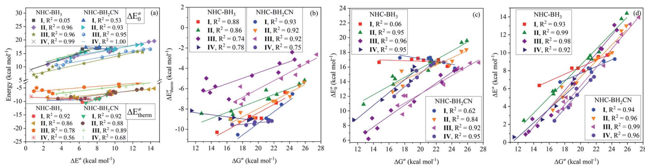
Fig. 6 Analysis of linear correlation degrees of activation barrier ( \Delta E^{\ddagger} ) to intrinsic barrier ( \Delta E_{\text{therm}}^{\ddagger} ) and thermal contribution ( \Delta E_{\text{therm}}^{\ddagger} ) (a) and of free energy barrier ( \Delta G^{\ddagger} ) to thermal contribution ( \Delta E_{\text{therm}}^{\ddagger} ) (b), intrinsic barrier ( \Delta E_{\text{therm}}^{\ddagger} ) (c), and activation barrier ( \Delta E^{\ddagger} ) (d).
