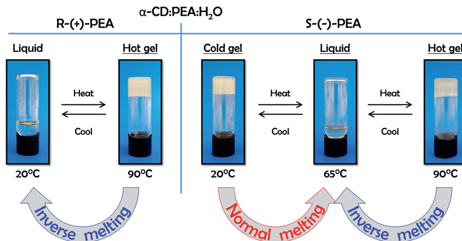
Fig. 1 Temperature dependent sol-gel phase transitions in \alpha CD/ R -PEA (left) and \alpha CD/ S -PEA (right) in the -10 to +100 °C temperature range.
