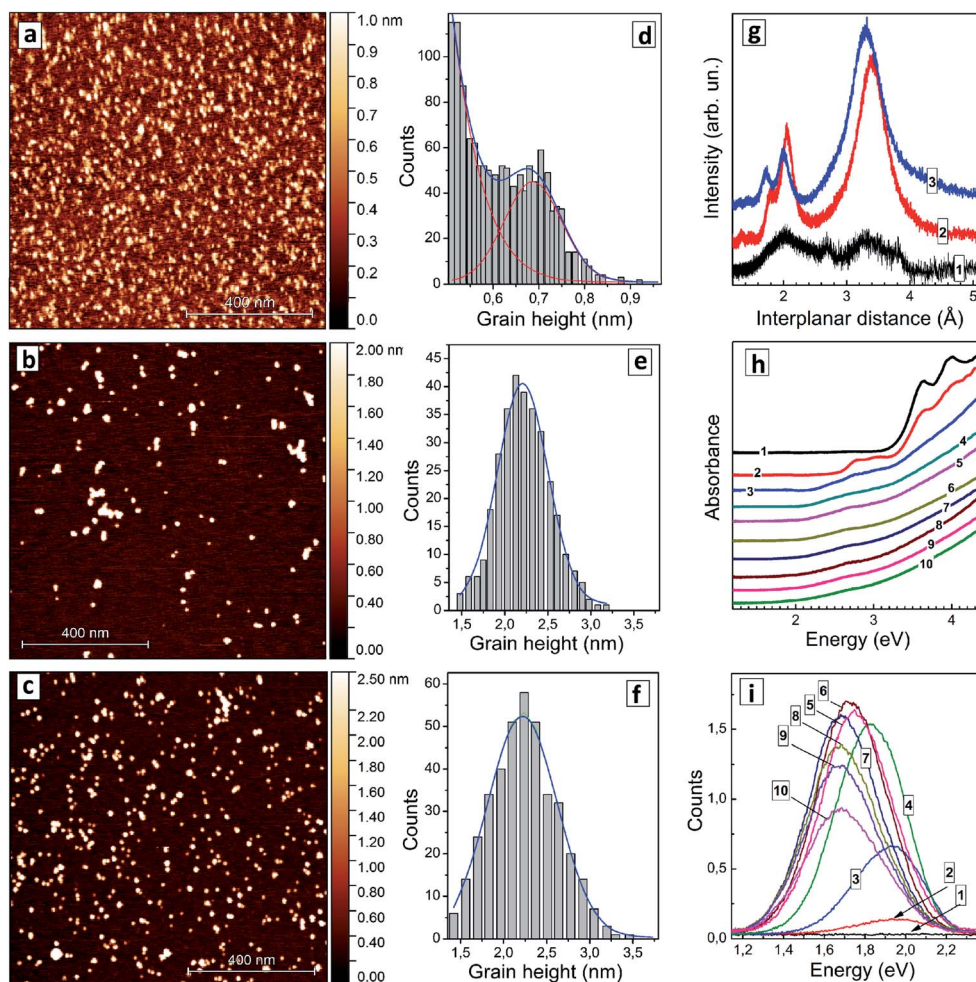
Fig. 1 (a–f) AFM images (a–c) and grain height distributions (d–f) of AISe QDs produced at nominal [\text{In}]/[\text{Ag}] ratio of 10 (a and d), 4 (b and e), and 2.7 (c and f). (g) XRD patterns of AISe QDs produced at [\text{In}]/[\text{Ag}] = 10 (curve 1) and 4 (curve 2). Curve 3 represents XRD pattern of Ag–In–S QDs produced at [\text{In}]/[\text{Ag}] = 4 . (h and i) absorption (h) and PL spectra (i) of AISe QDs produced at [\text{In}]/[\text{Ag}] = 0 (curves 1), 20 (2), 10 (3), 6.7 (4), 5 (5), 4.4 (6), 4 (7), 3.6 (8), 3.3 (9), and 2.7 (10).
