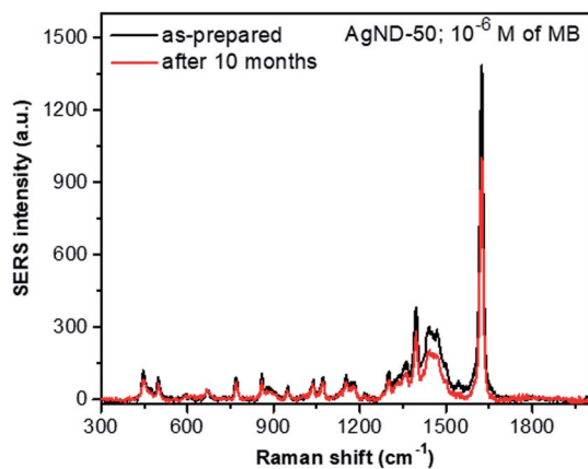
Fig. 14 The stability of SERS substrate based on AgND-50 with 10^{-6} M MB.
