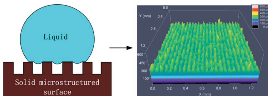
Fig. 5 "Cassie" contact state and three-dimensional topography of the sample surface after laser treatment.
