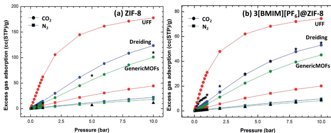
Fig. 3 Adsorption isotherm of (a) ZIF-8 and (b) 3[BMIM][PF 6 ]@ZIF-8 computed using different force fields in comparison with available experimental results ( \blacktriangle and \star represents experimental N 2 and CO 2 uptakes, respectively).
