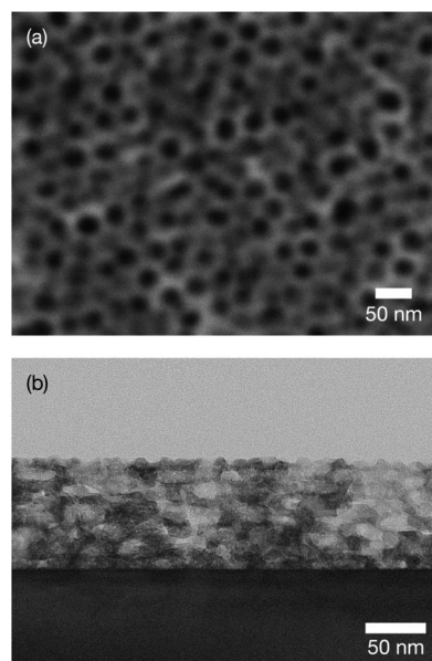
Fig. 1 (a) Top-view SEM and (b) cross-sectional TEM images of obtained mesoporous titania thin film on LAO substrate.
