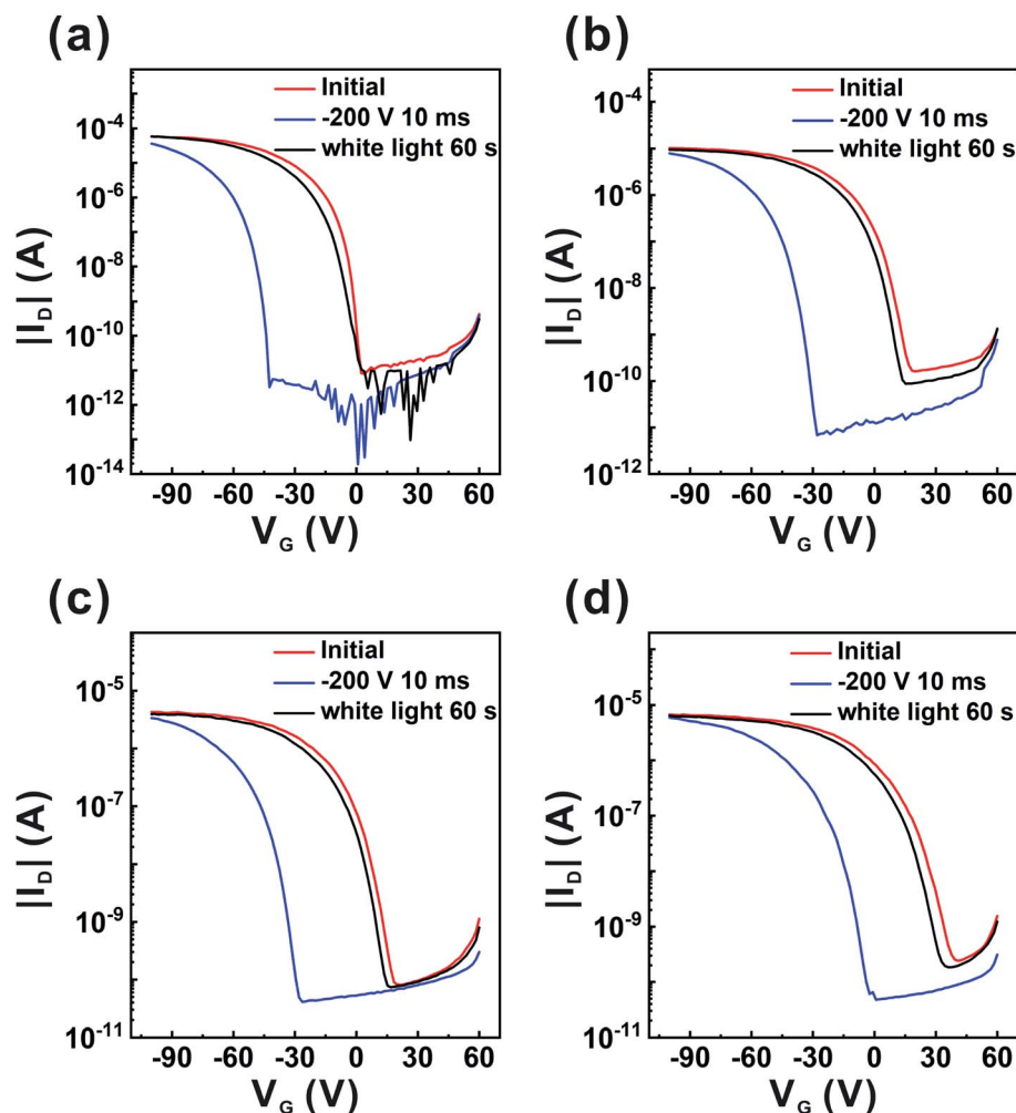
Fig. 2 Transfer characteristics ( V_D = -40 V) of the FGOFETMs based on pentacene with CPB QDs/PS composite floating-gate layers. (a) CPB QDs/PS = 1 : 1, (b) CPB QDs/PS = 3 : 1, (c) CPB QDs/PS = 4 : 1, (d) CPB QDs/PS = 6 : 1.
