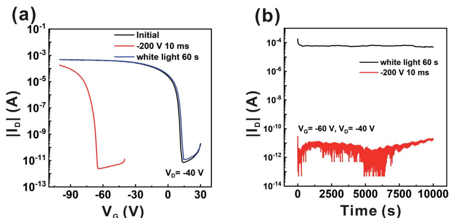
Fig. 3 (a) The transfer characteristics and (b) the retention characteristics of the FGO-FETMs based on C8-BTBT in electrical programming and photoinduced-reset states.
