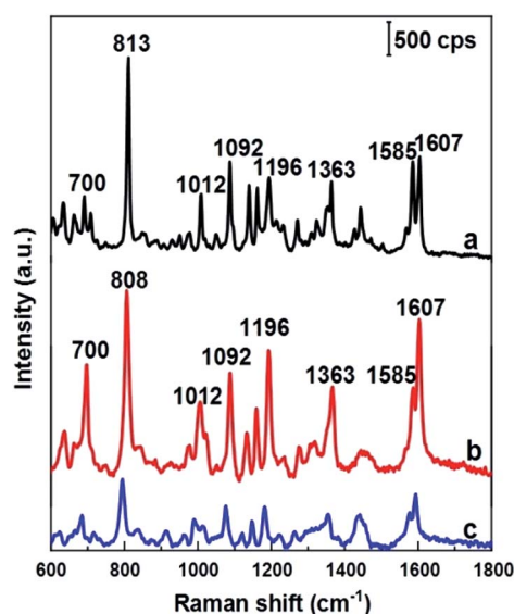
Fig. 4 Raman spectrum of DFC powder (a), and SERS spectra of 100 ppm DFC solution adsorbed on SERS substrates, which are AgNPs electrodeposited on silicon in either ethanol electrolyte (b) or aqueous electrolyte (c), provided that other conditions are the same ( 17^\circ\text{C} , 4 minutes, the electrolyte solution contains 0.1 mM \text{AgNO}_3 and 0.14 M HF, the current density is 0.3 \text{ mA cm}^{-2} ).
