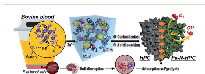
Fig. 1 Schematic for the synthetic process of the Fe–N–HPC electrocatalyst.
