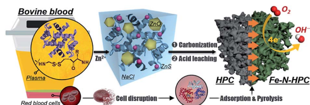
Fig. 1 Schematic for the synthetic process of the Fe–N–HPC electrocatalyst.
