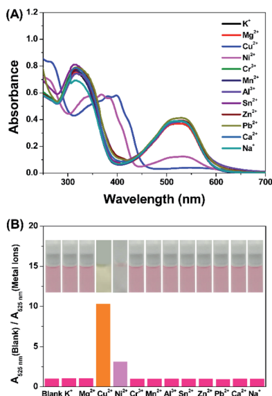
Fig. 3 (A) UV-vis absorption spectra of compound DTEP (10 μM) with various metal ions (40 μM) in MeOH solution after irradiation with 365 nm light. (B) The ratio of absorbance at 525 nm of compound DTEP (10 μM) without and with various metal ions (40 μM) in MeOH solution after irradiation with 365 nm light at 25 °C. Inset: the corresponding photographic images of compound DTEP with various metal ions (40 μM) after irradiation with 365 nm light.
