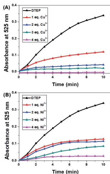
Fig. 4 Absorbance at 525 nm of compound DTEP (10 μM) with different amounts of Cu 2+ (A) and Ni 2+ (B) over irradiation time in MeOH solutions: none; 1 equiv.; 2 equiv.; 3 equiv. and 4 equiv.
