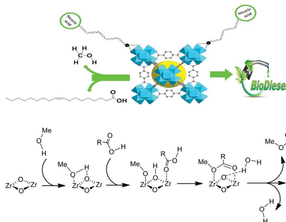
Scheme 1 Proposed scheme for the esterification of oleic acid over the 10% SA/UiO-66(Zr) catalyst.
