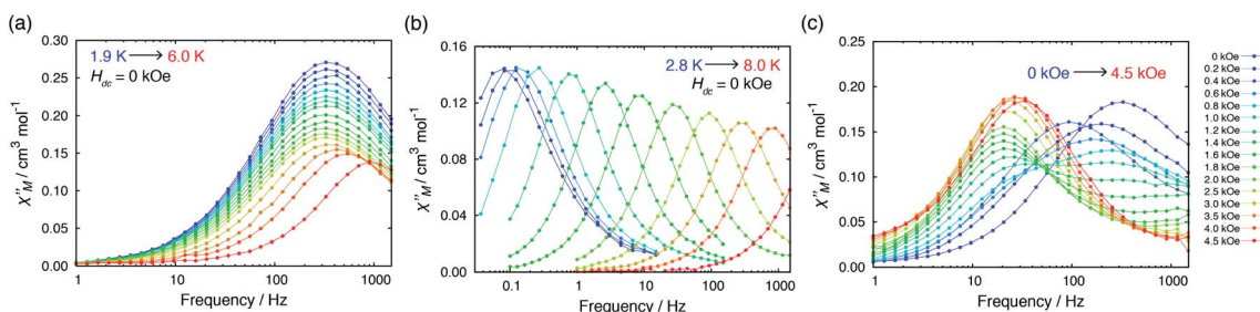
Fig. 4 Temperature dependence of out-of-phase ( \chi''_M ) susceptibilities for (a) 4·CH 3 OH and (b) 3'0.67 in the absence of the dc field. (c) Dc field-dependence of \chi''_M for 4·CH 3 OH with an dc field of 0–4.5 kOe.
