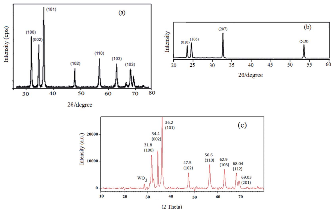
Fig. 4 Wide-angle XRD patterns of ZnO (a), \text{WO}_3 (b), and \text{WO}_3\text{ZnO}/\text{Fe}_3\text{O}_4 (c).
