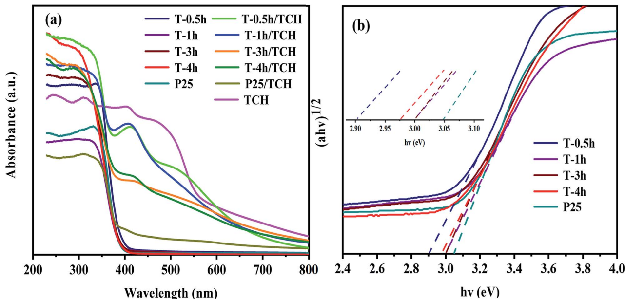
Fig. 7 (a) UV-Vis absorbance spectra of the samples and (b) the corresponding plots of (\alpha h\nu)^{1/2} versus h\nu .
