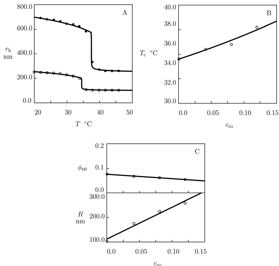
Fig. 4 (A) Hydrodynamic radius r_h of microgel particles versus temperature T . Symbols: experimental data 64 on P(NIPAm–TREGMA) microgels with molar fractions of comonomers c_{\text{cco}} = 0 (○) and c_{\text{cco}} = 0.12 (●). Solid lines: results of simulation. (B) Volume phase transition temperature T_c versus molar fraction of comonomers c_{\text{cco}} . Circles: experimental data. Solid line: results of simulation. (C) Parameters \phi_{n0} and R versus molar fraction of comonomers c_{\text{cco}} . Circles: treatment of observations. Solid lines: results of simulation.
