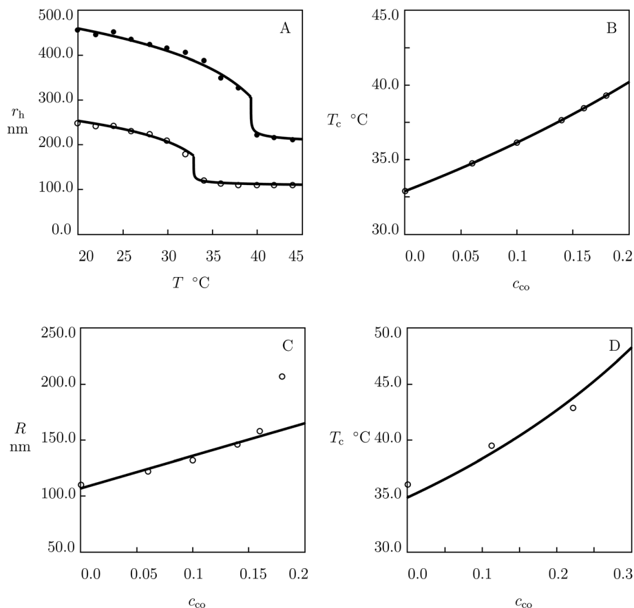
Fig. 6 (A) Hydrodynamic radius r_h of microgel particles versus temperature T . Symbols: experimental data 64 on P(NIPAm–DMAAm) microgels with molar fractions of comonomers c_{\text{co}} = 0 (○) and c_{\text{co}} = 0.18 (●). Solid lines: results of simulation. (B) Volume phase transition temperature T_c versus molar fraction of comonomers c_{\text{co}} . Circles: experimental data. Solid line: predictions of the model. (C) Radius R versus molar fraction of comonomers c_{\text{co}} . Circles: treatment of observations. Solid line: results of simulation. (D) Volume phase transition temperature T_c versus molar fraction of comonomers c_{\text{co}} . Circles: experimental data 57 on P(NIPAm–DMAAm) microgels. Solid line: predictions of the model.
