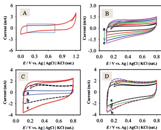
Fig. 5 CVs recorded for the GMCNT-15-modified electrode in the potential range from 0.0 to 1.2 V (A) at v of 10 mV s -1 and (B) in the potential range from 0.1 to 0.8 V at v of (a) 1, (b) 2, (c) 3, (d) 4 and (e) 5 mV s -1 . (C) CVs measured for (a) F-MWCNT, (b) GOM, (c) GMCNT-15 and (D) for (a) GMCNT-5, (b) GMCNT-10, (c) GMCNT-30, (d) GMCNT-50 composite-modified electrodes at v of 10 mV s -1 . The electrolyte solution was an aqueous 0.5 M Na 2 SO 4 solution.
