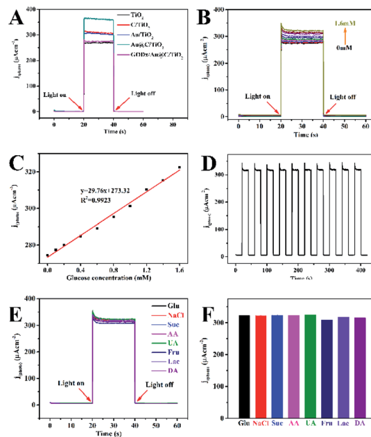
Fig. 7 (A) The j(\text{photo}) – t responses of \text{TiO}_2 , \text{C}/\text{TiO}_2 , \text{Au}/\text{TiO}_2 , \text{Au}@/\text{C}/\text{TiO}_2 and \text{GODx}/\text{Au}@/\text{C}/\text{TiO}_2 in 0.1 M pH 7.4 PBS at 0.4 V vs. \text{Ag}/\text{AgCl} , (B) the j(\text{photo}) – t responses of \text{GODx}/\text{Au}@/\text{C}/\text{TiO}_2 toward Glu at increasing concentration from 0 mM to 1.6 mM in the supporting electrolyte of 0.1 M pH 7.4, (C) linear calibration ([Glu] vs. j(\text{photo}) ) curve, (D) Stability of \text{GODx}/\text{Au}@/\text{C}/\text{TiO}_2 electrode with 1.6 mM glucose, (E and F) Effect of interferences on the response photocurrents. Experiments were performed in 0.1 M pH 7.4 PBS containing 1.6 mM of Glu with NaCl, Suc, AA, UA, Fru, Lac and DA with light ON.
