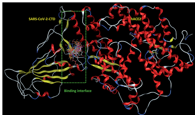
Fig. 2 Overlay of 1 (cyan sticks), 2 (yellow sticks), 3 (magenta sticks), 4 (orange sticks), 6 (light pink sticks), 7 (green sticks), 8 (deep pink sticks), 9 (white sticks), 10 (red sticks), 11 (deep yellow sticks), 12 (pink sticks) and 13 (blue sticks) in the binding interface of SARS-CoV-2-CTD in complex with hACE2 (PDB ID 6LZG).
