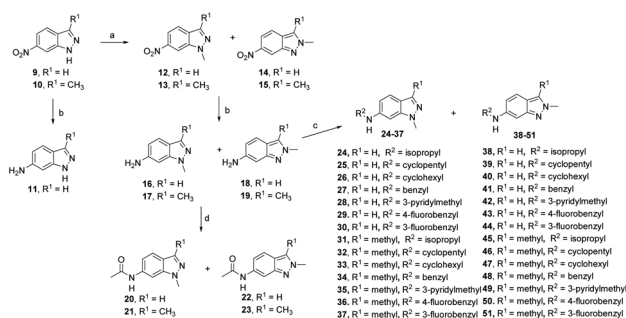
Scheme 1 Reagents and conditions: (a) CH_3I (2.0 equiv.), excess K_2CO_3 , DMF, 60 °C, 4 h, 95–98%; (b) H_2 , Pd/C (10 mol%), r.t., 4 h, 85–96%; (c) ketone or aldehyde (1.0 equiv.), NaBH_3CN (5.0 equiv.), AcOH, MeOH, 40 °C, 4 h, 73–96%; (d) excess Ac_2O , TEA, DMC, r.t., 2 h, 89–92%.
