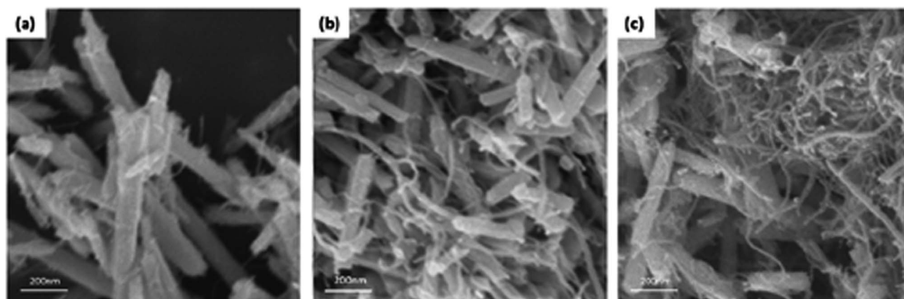
Fig. 8 FE-SEM images of MWCNT/Te nanorod composites with various MWCNT contents (a) 1 wt%, (b) 3 wt%, and (c) 5 wt%.
